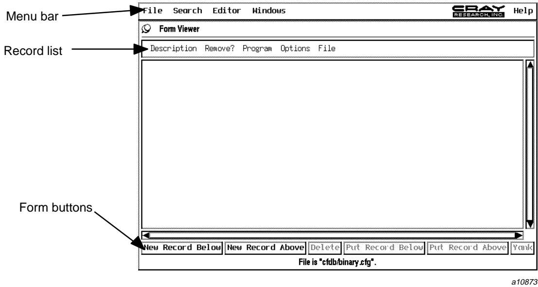
Figure 8. Form menu
