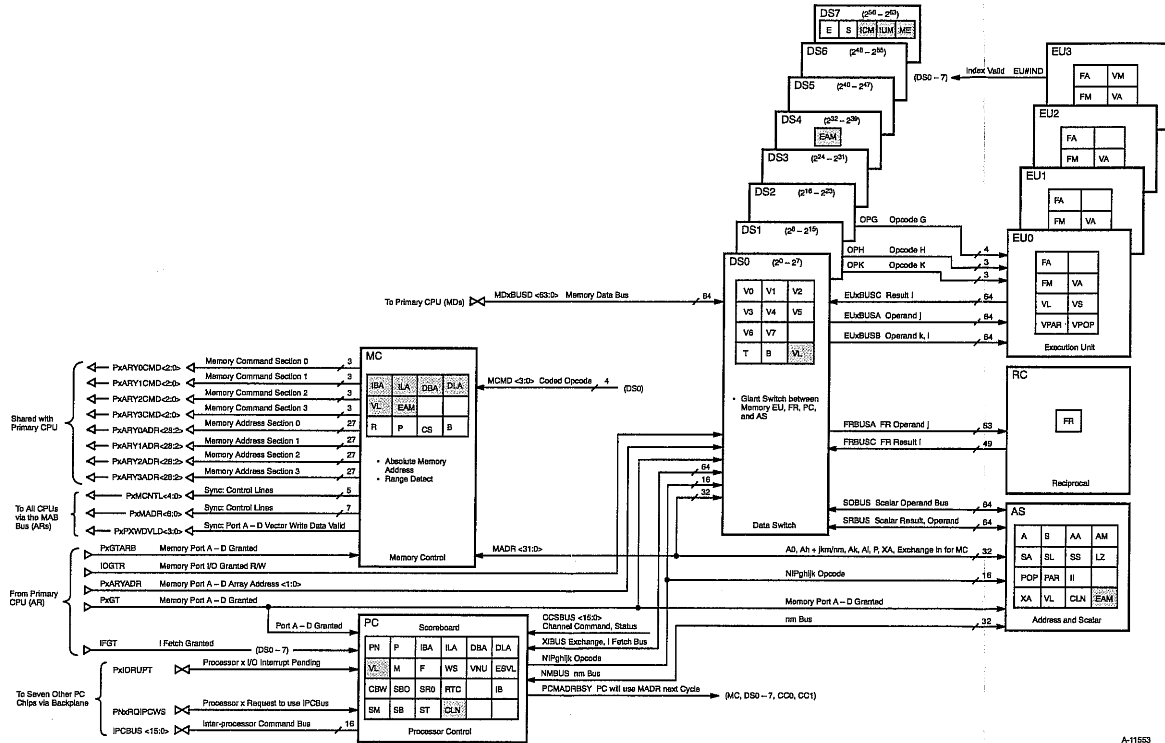
Figure 2-3. Secondary CPU Bus Block Diagram
