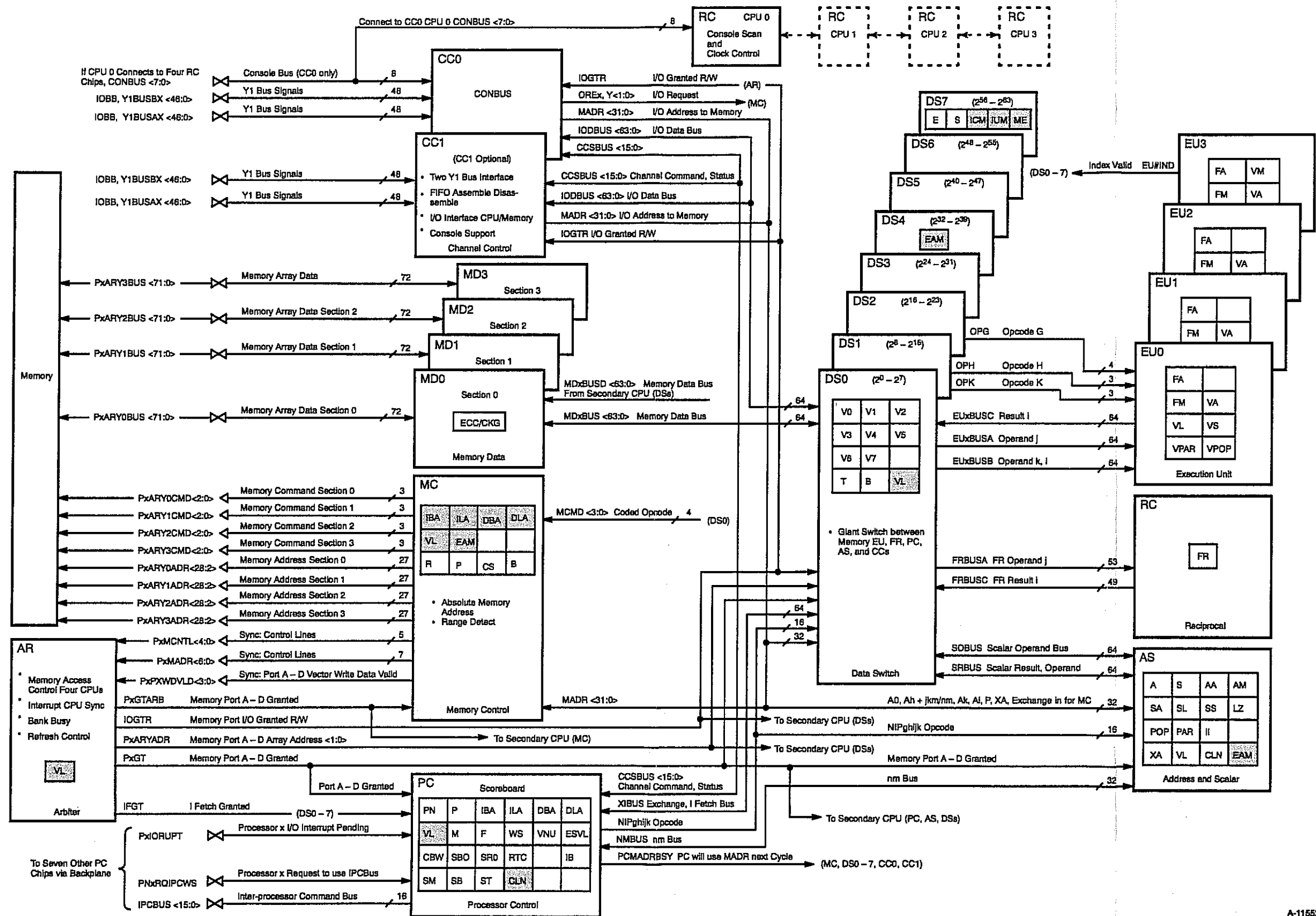
Figure 2-2. Primary CPU Bus Block Diagram
