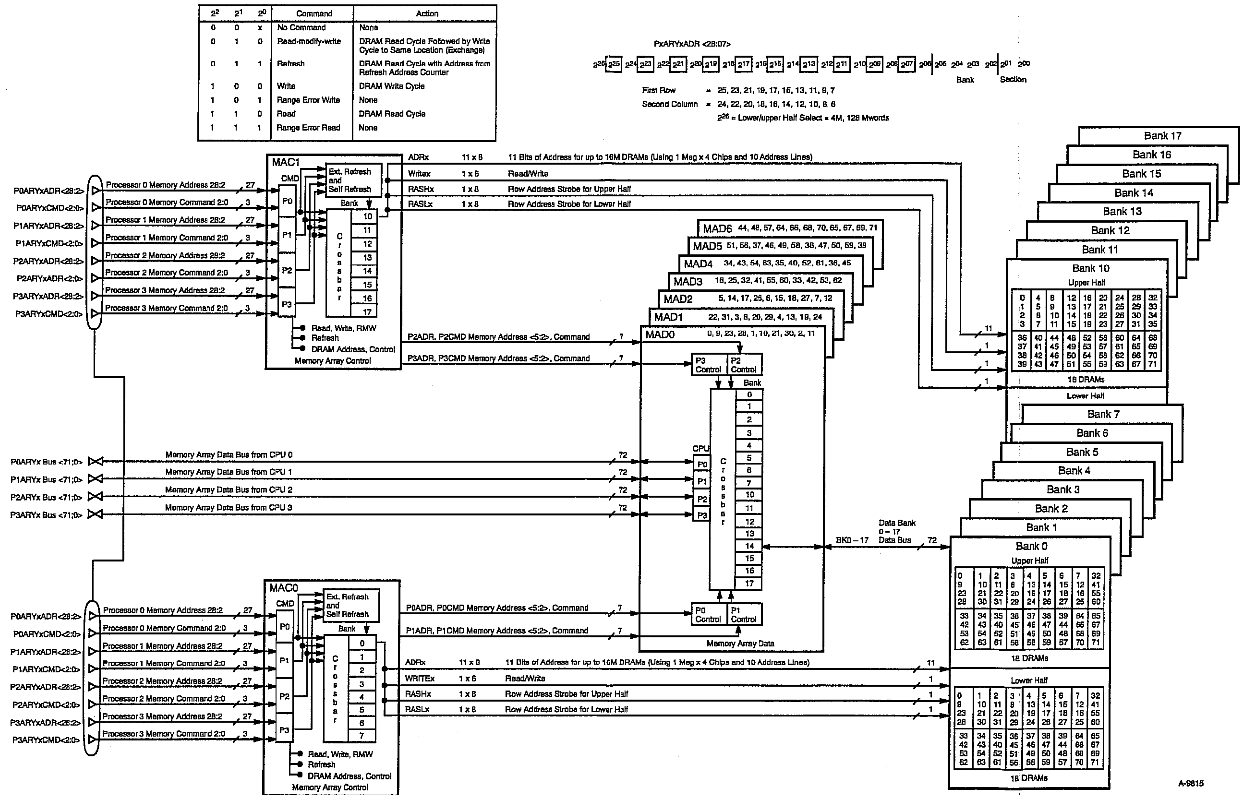
Figure 3-4. Memory Block Diagram
