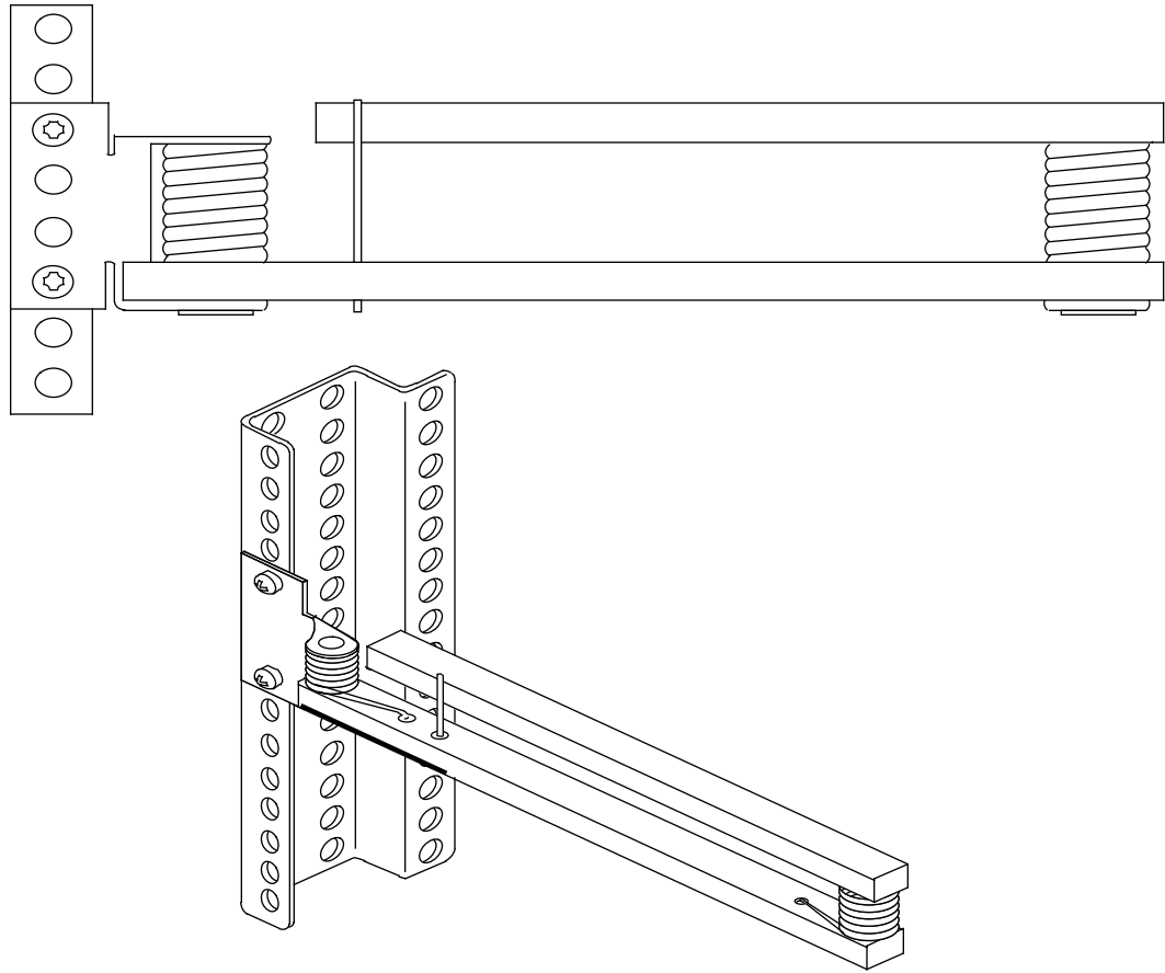
Figure 5. Cable Retractor
