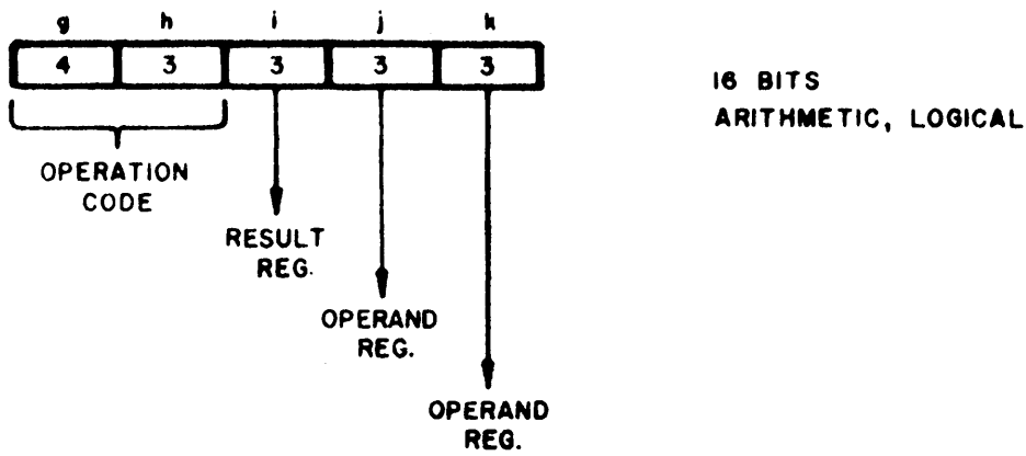
Figure 4-2. Format for arithmetic and logical instructions
