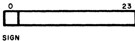
2's COMPLEMENT INTEGER (24 BITS)
