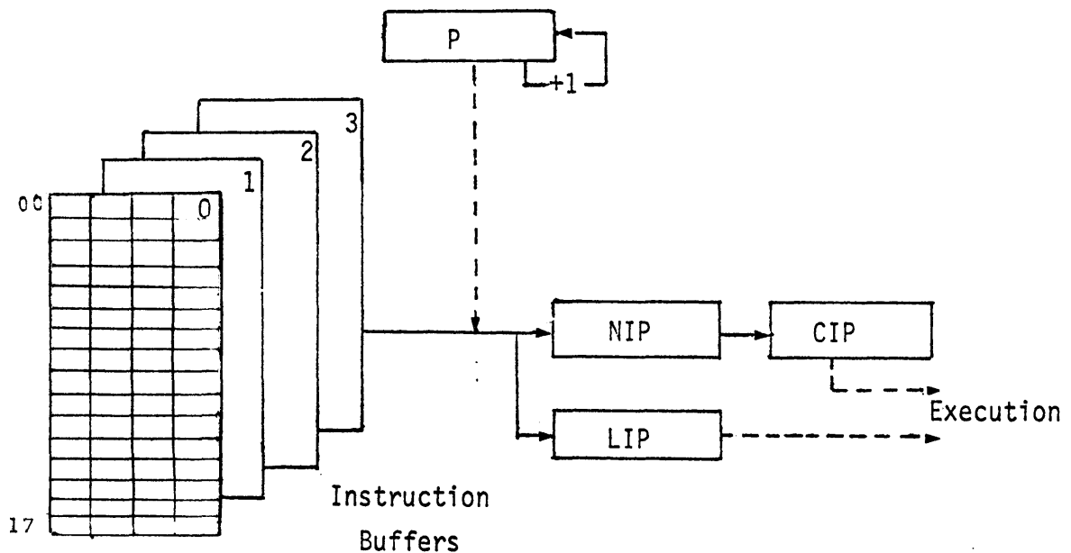
Figure 3-6. Relationship of instruction buffers and registers
