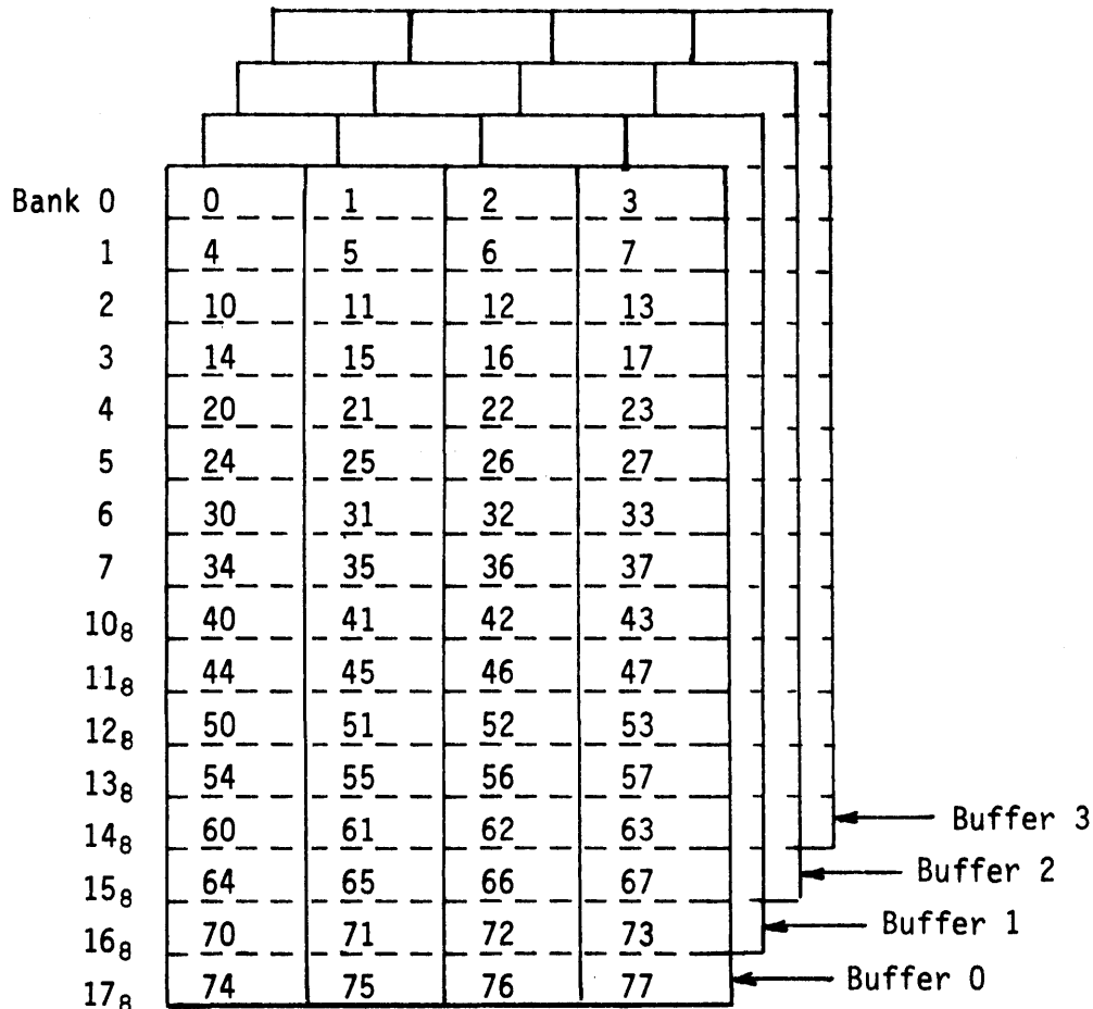
Figure 3-7 Instruction buffers
