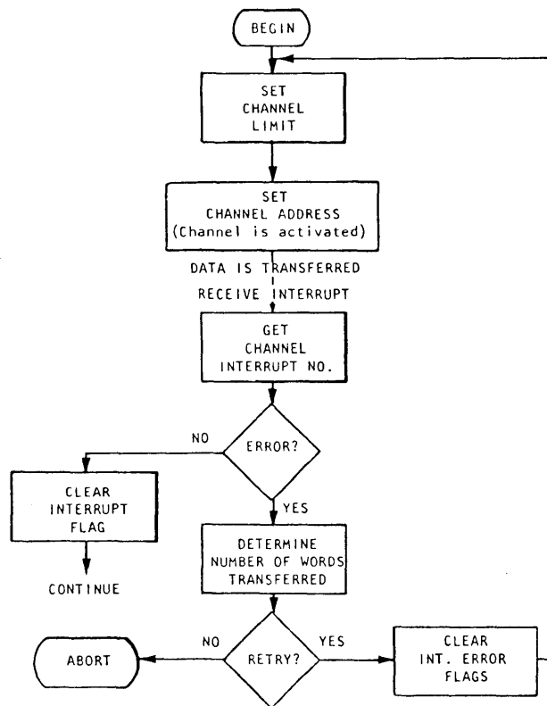
Figure 6-1. Basic I/O program flow chart
