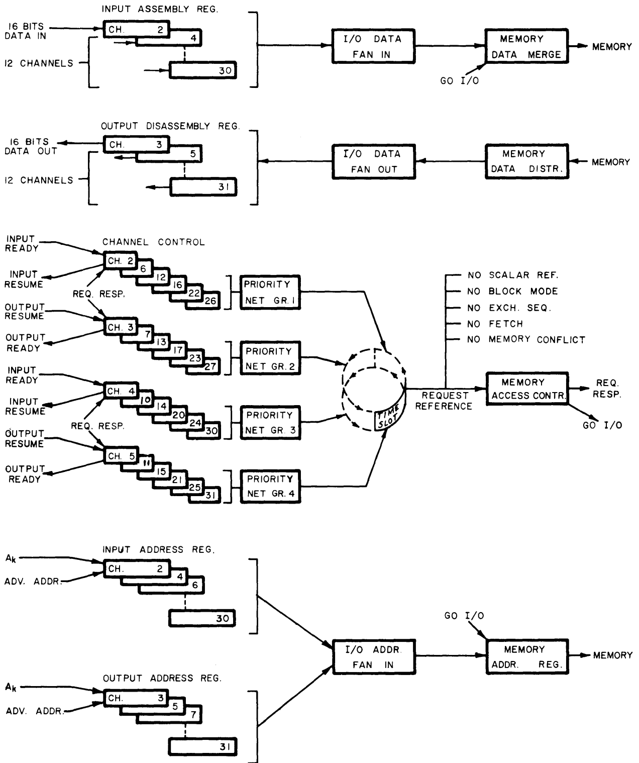
Figure 6-2. Channel I/O control
