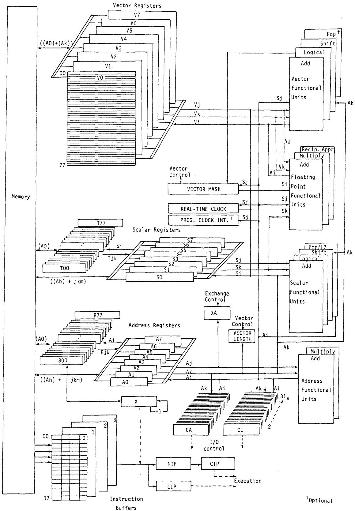
Figure 3-1. Computation section
