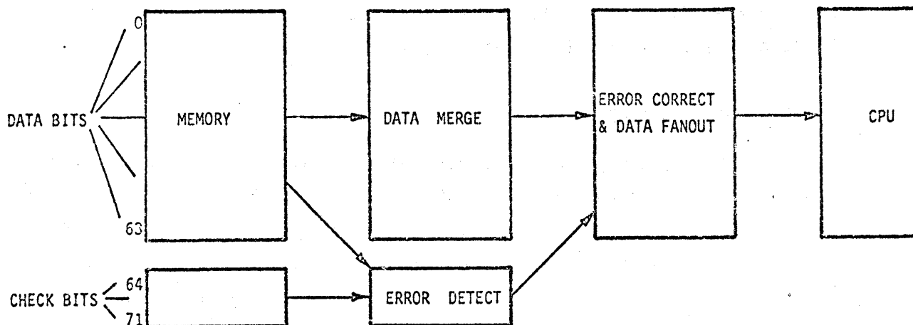
Figure 5-2. Memory data path with SECDED
