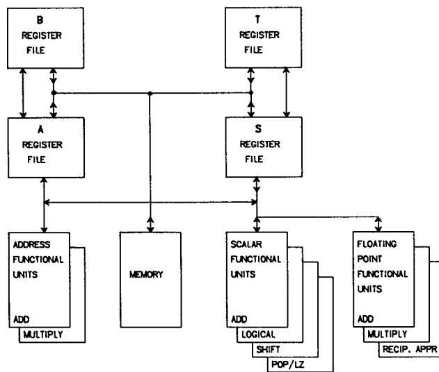
Figure 1 -- The CRAY-1 Scalar Architecture
