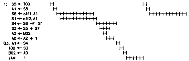
(b) The CRAY-1
