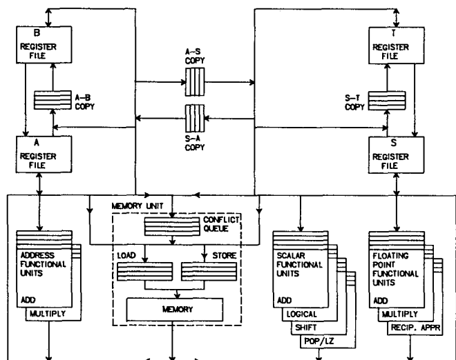
Figure 3 -- A modified CRAY-1 scalar architecture to issue instructions out-of-order.
