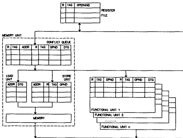
Figure 2 -- Tag based mechanism to issue out-of-order.
