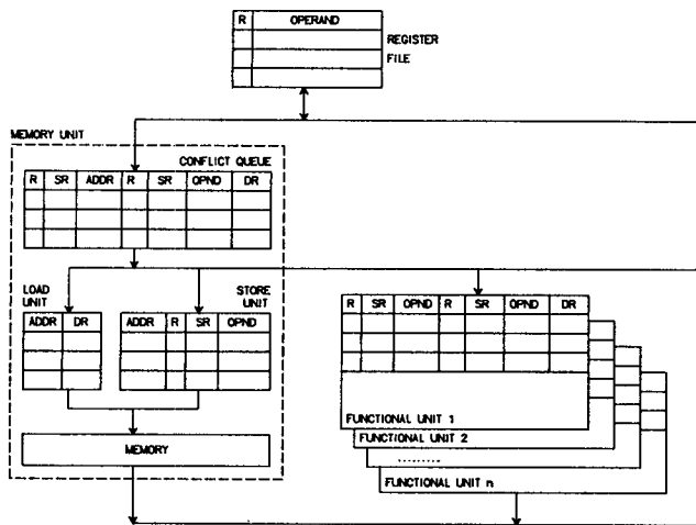
Figure 5 -- Thornton's issue logic.
