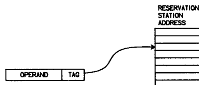
Figure 6 -- Tag Search Table for the DTS Algorithm.
