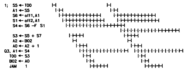
(c) Tomasulo's algorithm
