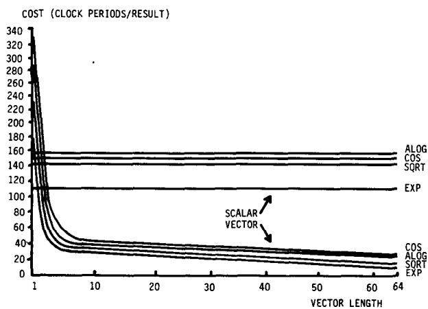
Fig. 7. Scalar/vector timing.
