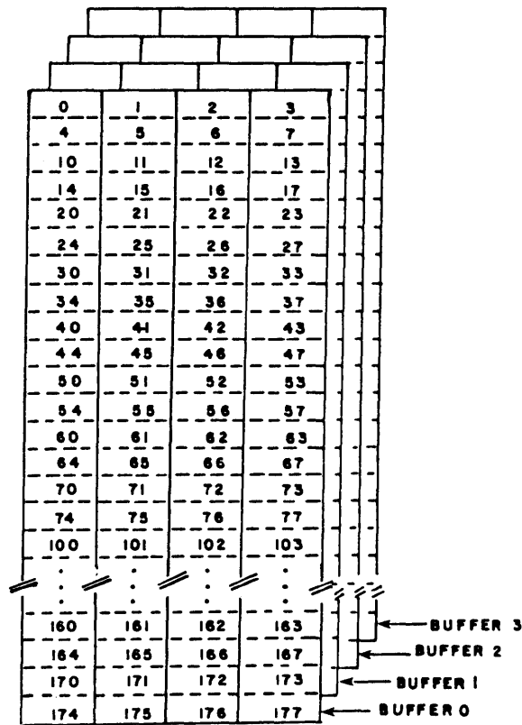
Figure 3-2. Instruction buffers
