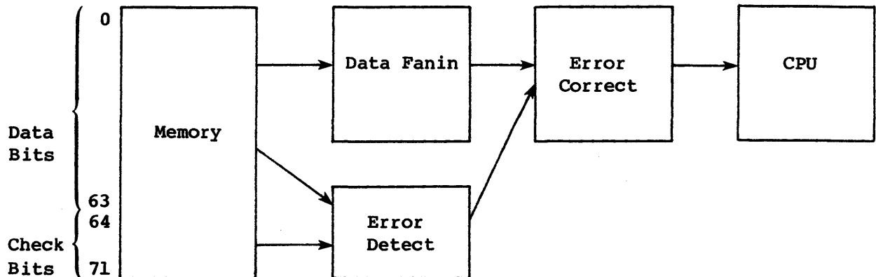
Figure 2-6. Memory data path with SECDED
