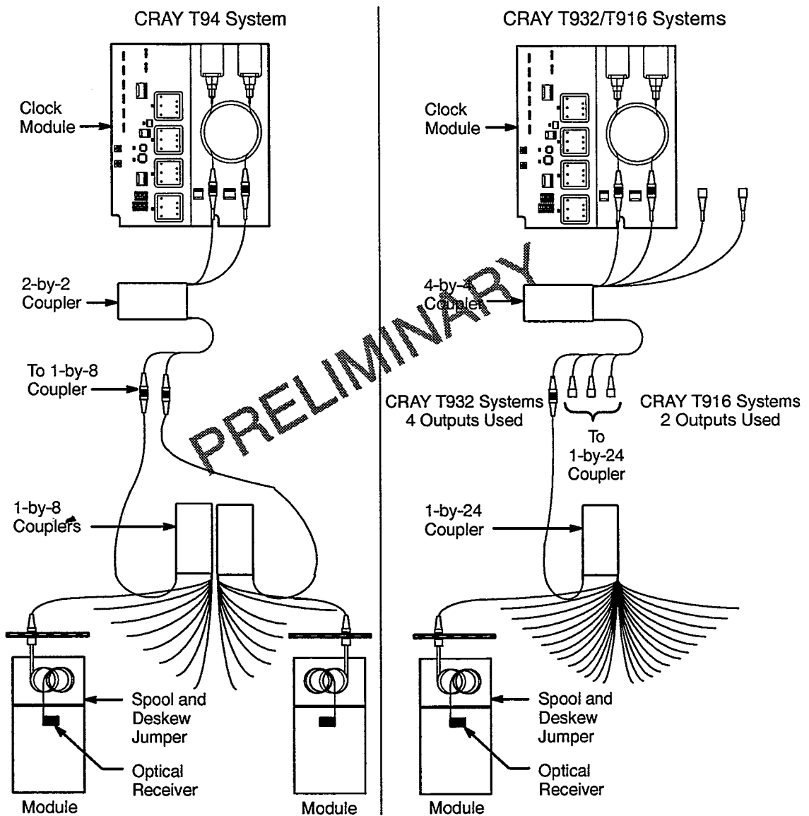
Figure 11. Optical Clock Path
