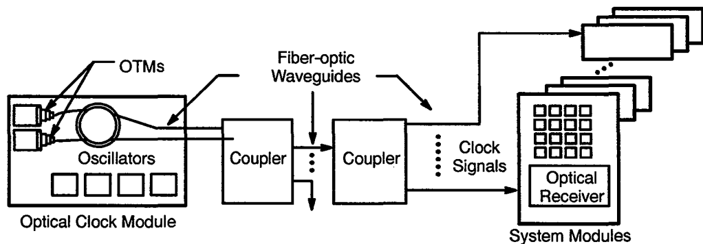
Figure 1. Optical Clock Signal Path
