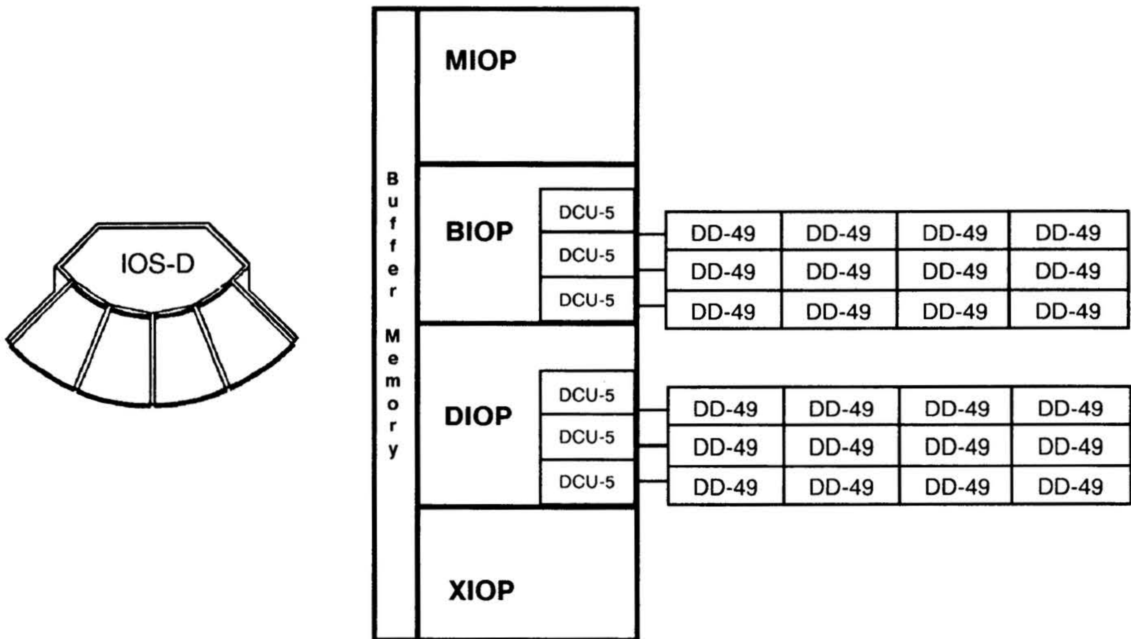
IOS Model D and DD-49 Disk Drive Maximum Configuration
