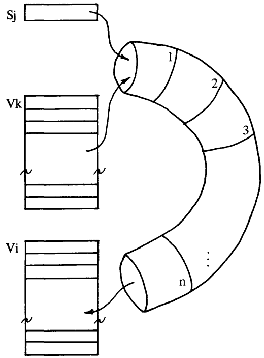
Figure 2b. Type II vector instruction
